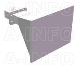
LB-430-15-C-SFSPO Standard Gain Horn Antenna 1.7-2.6GHz 15dB Gain SMA Female
